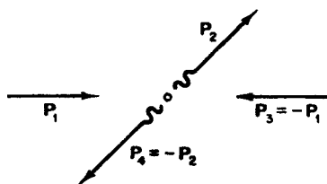
FIGURE V.2 Scattering when \mathbf{P} = 0 .
