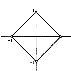
FIGURE IV.2 The unit sphere in \mathbb{R}^2 when \|(x, y)\| = |x| + |y| .
